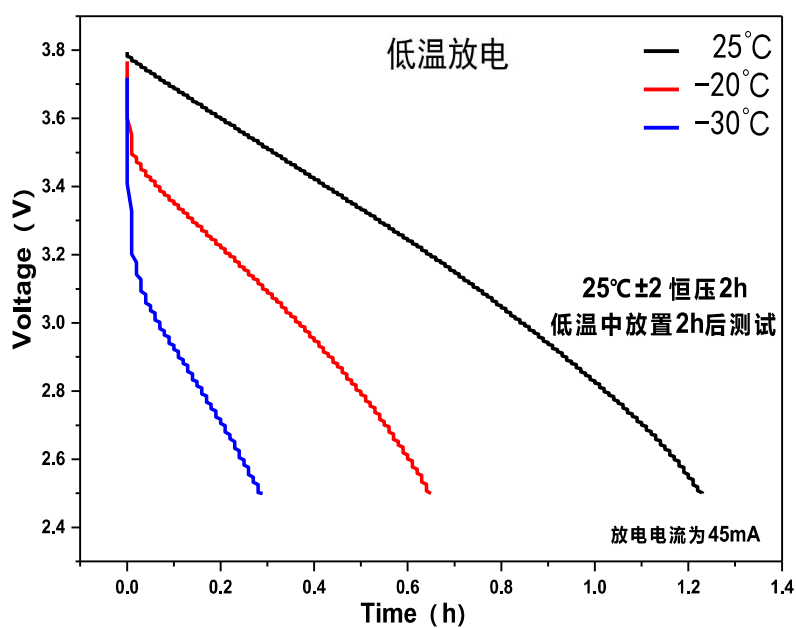
低温放电容量变化 Capacitance changes at low temp. discharge condition
