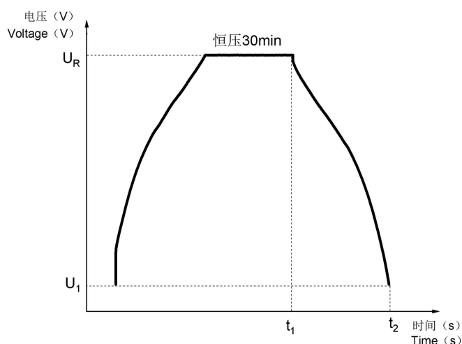
Fig1. Charge/Discharge curves for Sample
